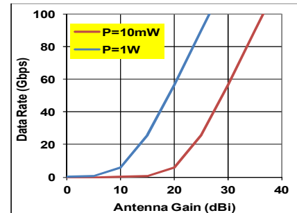
Figure 7. The maximum achievable data rates for the interior WLAN applications with 10mW or 1W transmit power.
